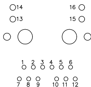
PIN ASSIGNMENTS (COMPONENT SIDE VIEW)
