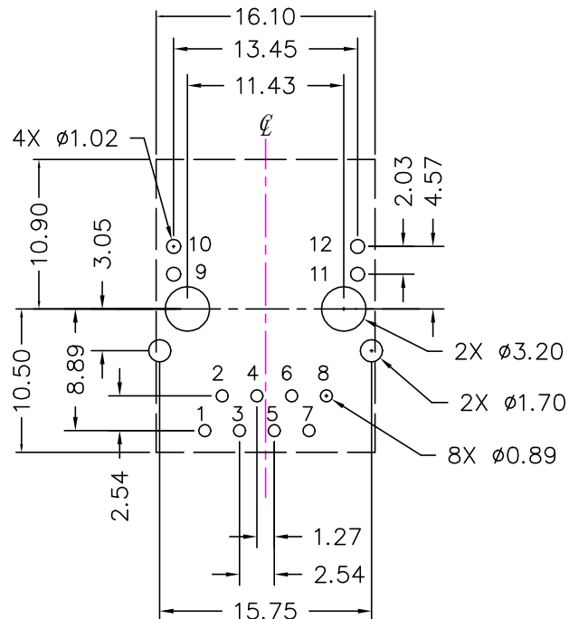
Recommended PCB layout (Component Side View)
