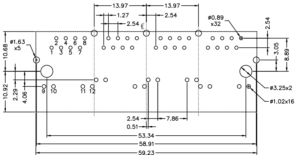
Recommended PCB layout (Component Side View)
