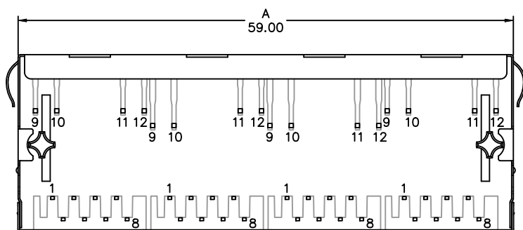
(Bottom View)
