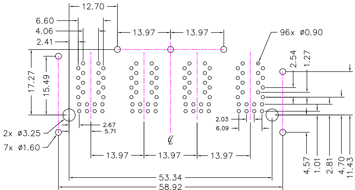
Recommended PCB layout (Component Side View)
