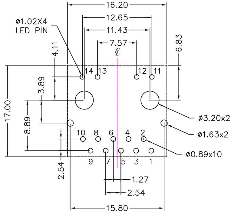
Recommended PCB layout (Component Side View)
