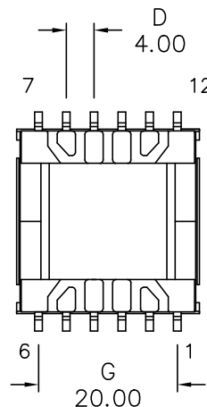
(Bottom View)
